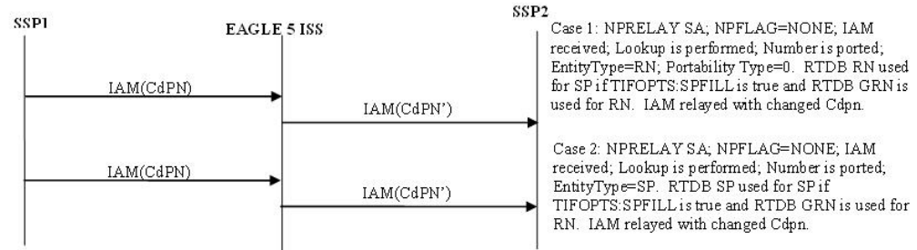
Figure 3-8 ISUP Message Flows for Service Portability
