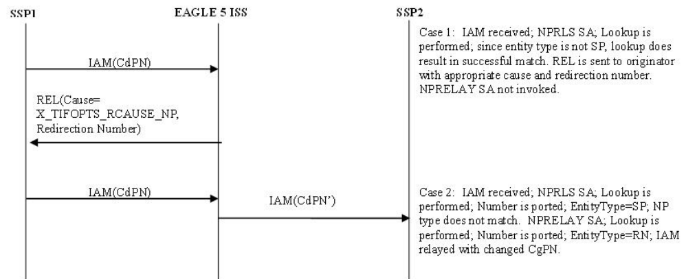
Figure 3-9 ISUP Message Flows for NPRLS + NPRELAY
