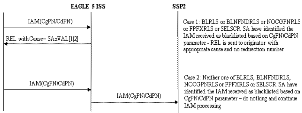
Figure 3-25 TIF Blocklist Basic Message Flow
